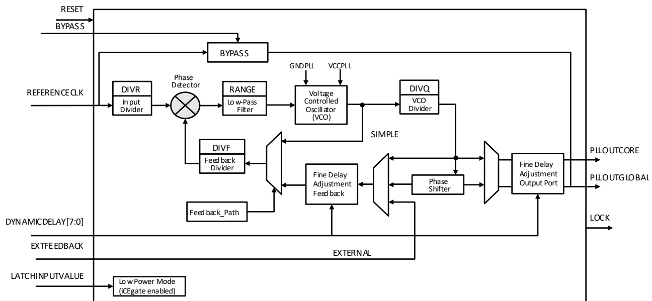
Figure 3.3. PLL Diagram
