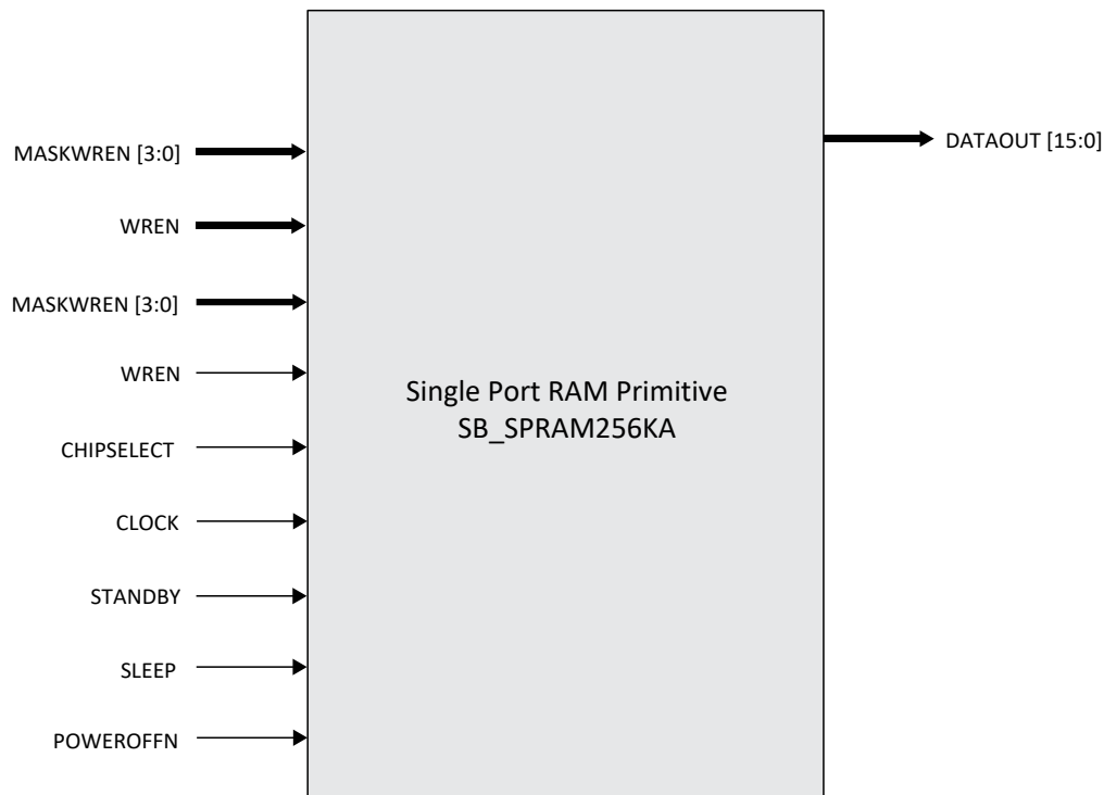
Figure 3.5. SPRAM Primitive
